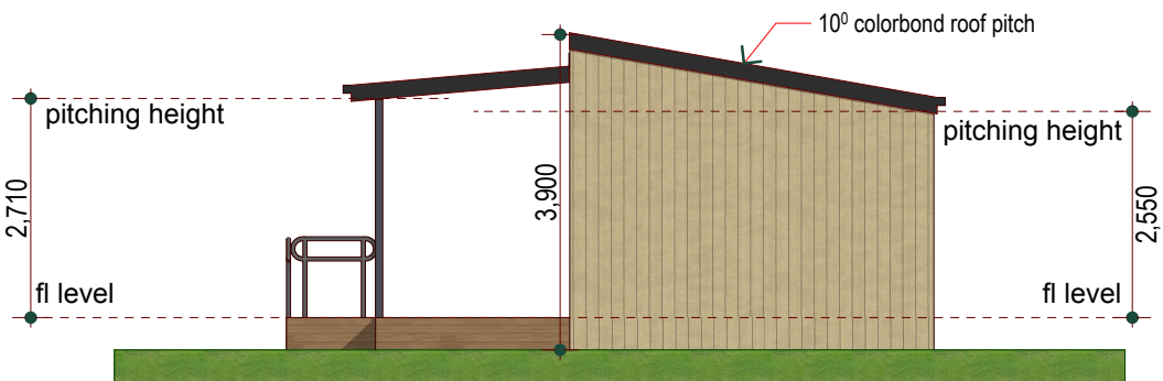
side elevation
